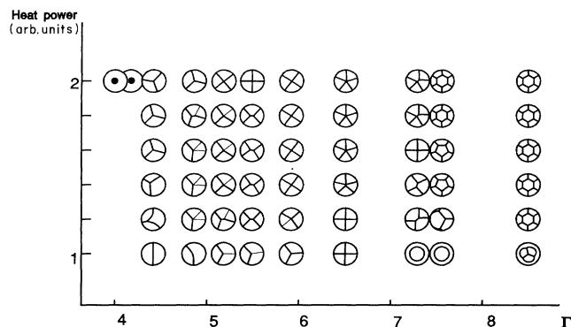
FIG. 3. Schematic representation of the stationary patterns observed in the experiments for different aspect ratios and heating. In the first two patterns, dark points correspond to upflow motions. In the rest of the patterns, cold lines are represented by solid lines.
