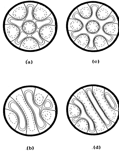
FIG. 10. When \delta is decreased the roll solution is recovered. (a) \Gamma = 6.5 , \delta = 1 ; (b) \Gamma = 6.5 , \delta = 0 ; (c) \Gamma = 7.3 , \delta = 1 ; (d) \Gamma = 7.3 , \delta = 0 . ( \epsilon = 0.5 .)
