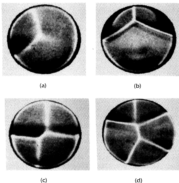
FIG. 4. Shadowgraphs of nonsymmetrical patterns.
