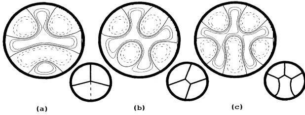
FIG. 8. Contour plots of nonsymmetric patterns. (a) \Gamma = 5.5 , \epsilon = 0.3 , (b) \Gamma = 5.8 , \epsilon = 0.3 , (c) \Gamma = 6 , \epsilon = 0.5 .
