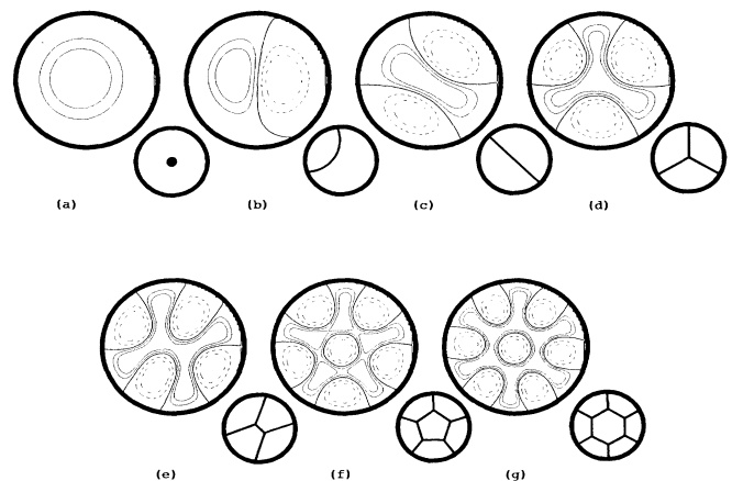
FIG. 7. Contour plots for stable amplitude field \Psi(x, y) . Five contour lines are drawn that correspond to -M/2 , -M/4 , 0 , M/4 , and M/2 , where M is the maximum of \Psi . At the bottom right of each figure shows the pattern that would be seen with a shadow-graph system. Aspect ratios are (a) \Gamma=2.4 , (b) \Gamma=3.5 , (c) \Gamma=3.8 , (d) \Gamma=4.5 , (e) \Gamma=5.7 , (f) \Gamma=6.5 , and (g) \Gamma=7.3 ( \epsilon=0.5 ).
