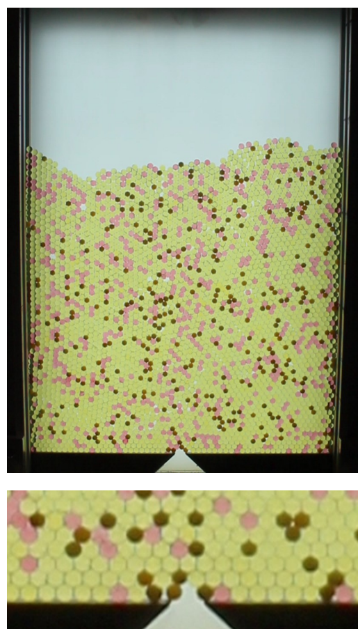
Fig. 1 Top: Image of the container filled with a mixture with 10 % hard frictional beads. Yellow and pink colored hydrogel spheres are equivalent, airsoft bullets appear dark. Bottom: Zoom into the region near the orifice at the bottom, in a clogged state. The orifice in these images is D = 11 mm, slightly less than two particle diameters.
