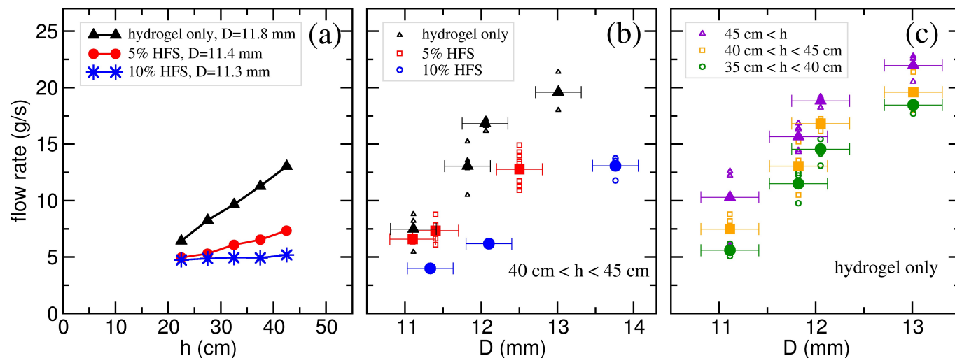
Fig. 5 (a) Flow rate as a function of the bed height h for pure hydrogel and for mixtures with 5% and 10 % HF spheres. (b) Flow rate as a function of orifice size D for all 3 samples for a bed height of 40 \text{ cm} < h < 45 \text{ cm} and for (c) pure hydrogel samples at various bed heights h . Small open symbols represent individual experiments, large filled symbols show averages of the respective data sets (on average 4 experiments).
