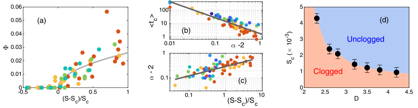
FIG. 3. (a) \Phi vs the supercriticality (S - S_c)/S_c , for D = 2.3, 2.6, 2.8, 3.2 [same colors as Fig. 2(a)]. The gray line corresponds to the expression \Phi \sim [(S - S_c)/S_c]^{1/2} ; see text. (b) \langle t_c \rangle divergence at \alpha = 2 . (c) \alpha - 2 as a function of supercriticality. The solid lines are the algebraic fittings explained in the text. (d) S_c for the different orifice sizes tested, delimiting the boundary between clogged and unclogged states in the plane S - D .
